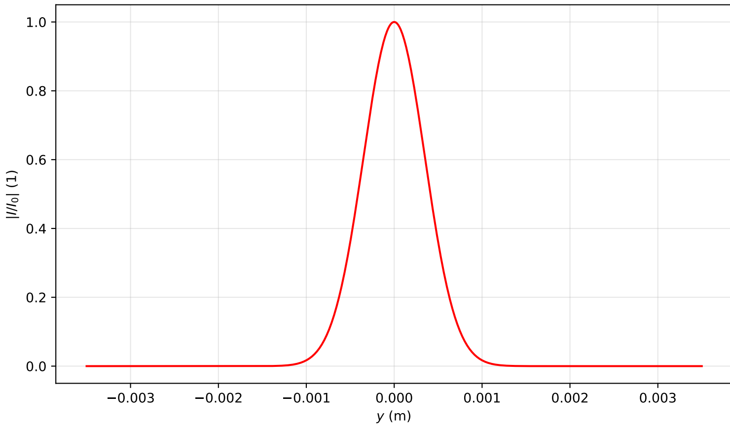
Intensity profile I(x = 0, y, z = 0.000)/I_0 , P_{in}=6.5P_{cr} , artificial time
